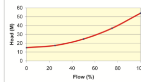
Figure 7.2 System Resistance Curve
