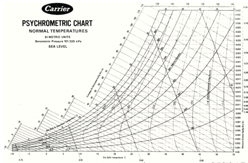
Figure 9.1 Psychrometric Chart
